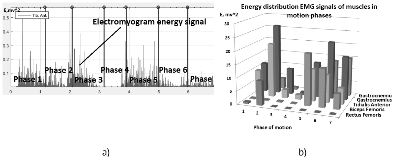
Figure 7. Amplitude-time analysis of EMG signals of muscles: a - EMG-signals' energy of the muscle Tibialis Anterior of the right leg when doing the motion test 1; b - the energy distribution of the EMG signals of the right leg's muscles in the phases of movement during the motion test 1.
