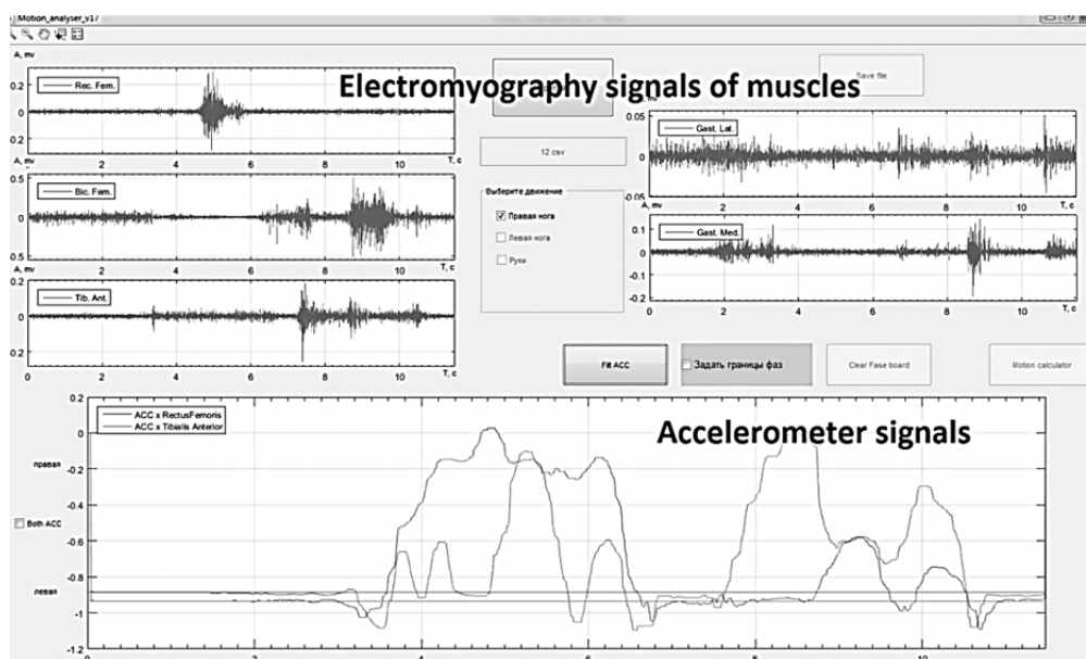
Figure 5. Interface of the program "Motion analyzer".
